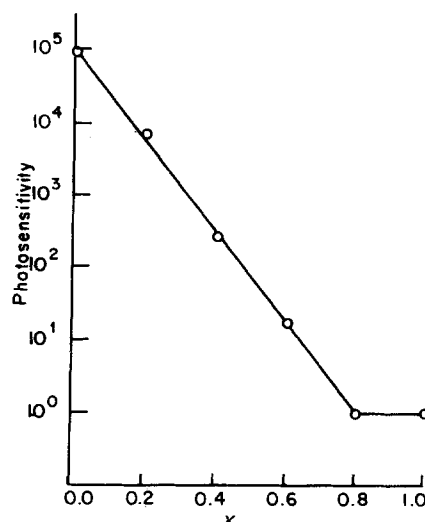
Figure 6 Photosensitivity (photoconductivity/dark conductivity) against x for Zr_xCd_{1-x} films.
