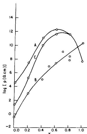
Figure 5 Variation of logarithm of resistivity with x for (A) screen-printed and sintered film of Zr_xCd_{1-x}S , (B) vacuum-evaporated Zr_xCd_{1-x}S thin film [1], and (C) Film (A) annealed in H_2 at 200^\circ C for 30 min.
