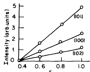
Figure 3 Variation of intensity of X-ray diffraction lines (100), (101) and (102) belonging to zinc.
