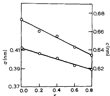
Figure 2 Variation of lattice parameters a and c of Zr_xCd_{1-x}S solid solutions.
